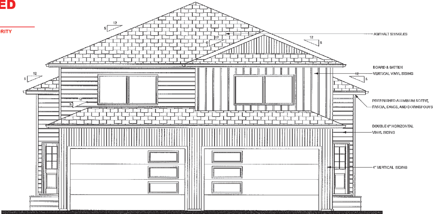
FRONT ELEVATION
